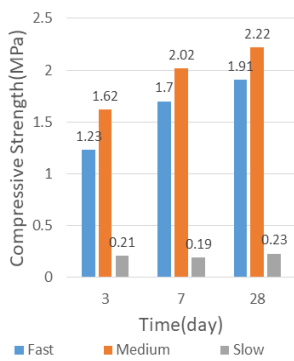
Fig. 4. K.G.O-IG Compression strength
