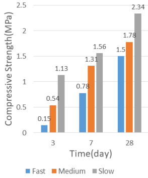
Fig. 2. K.G.O-CG Compression strength
