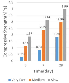
Fig. 3. K.G.O-CH Compression strength
